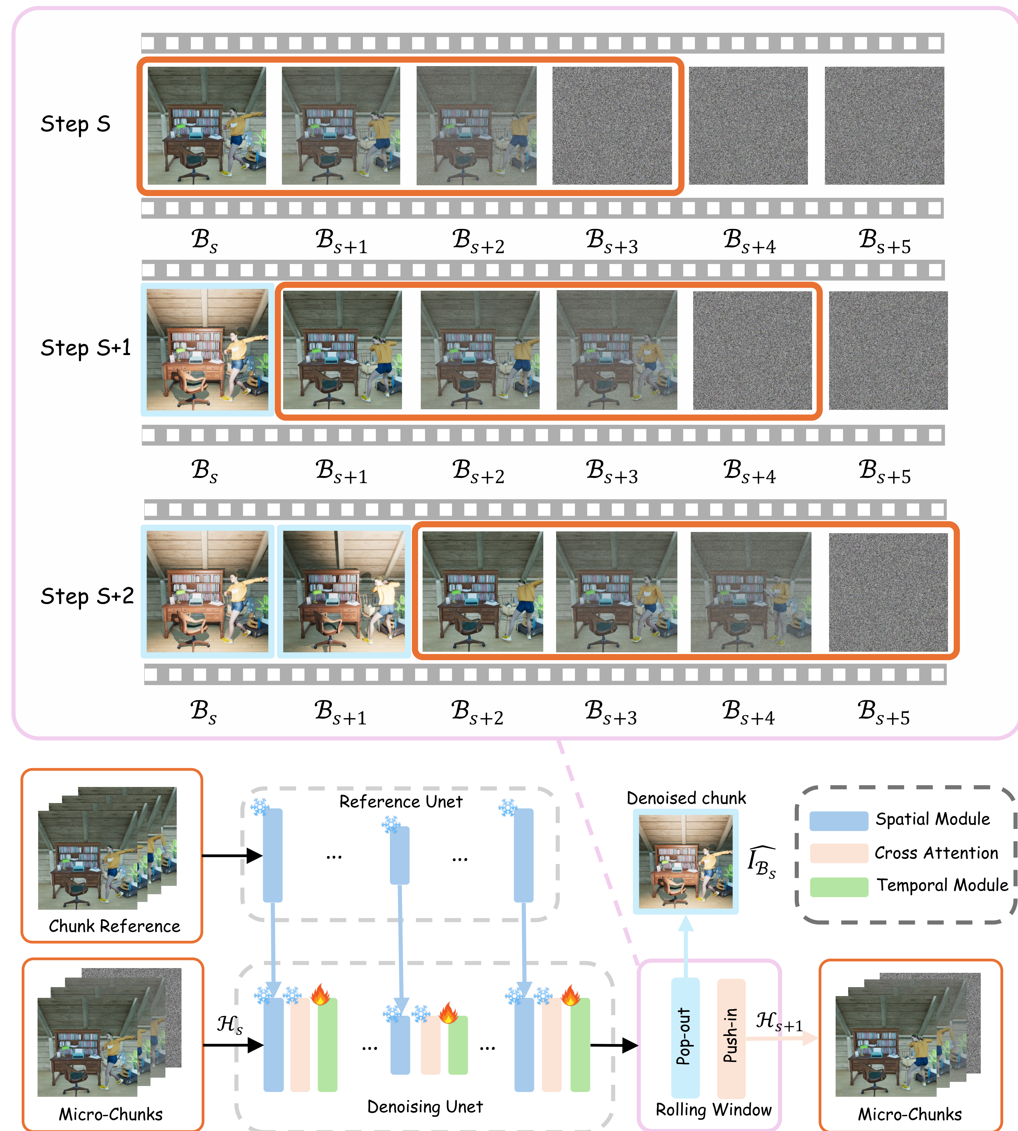
(c) Rolling-Window Streaming Video Relighting
