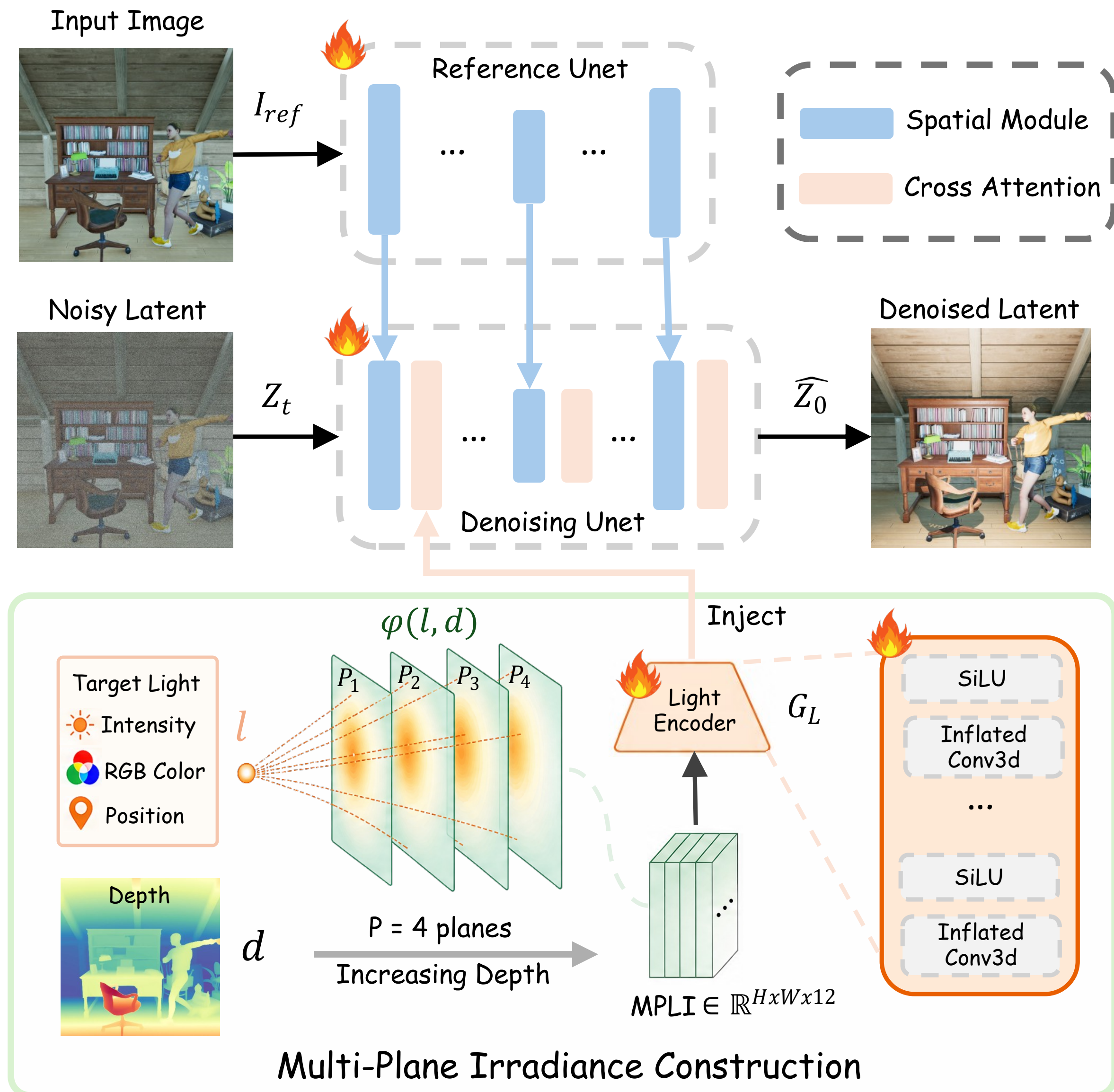
(a) Lightweight Multi-Plane Lighting Interactive Control
