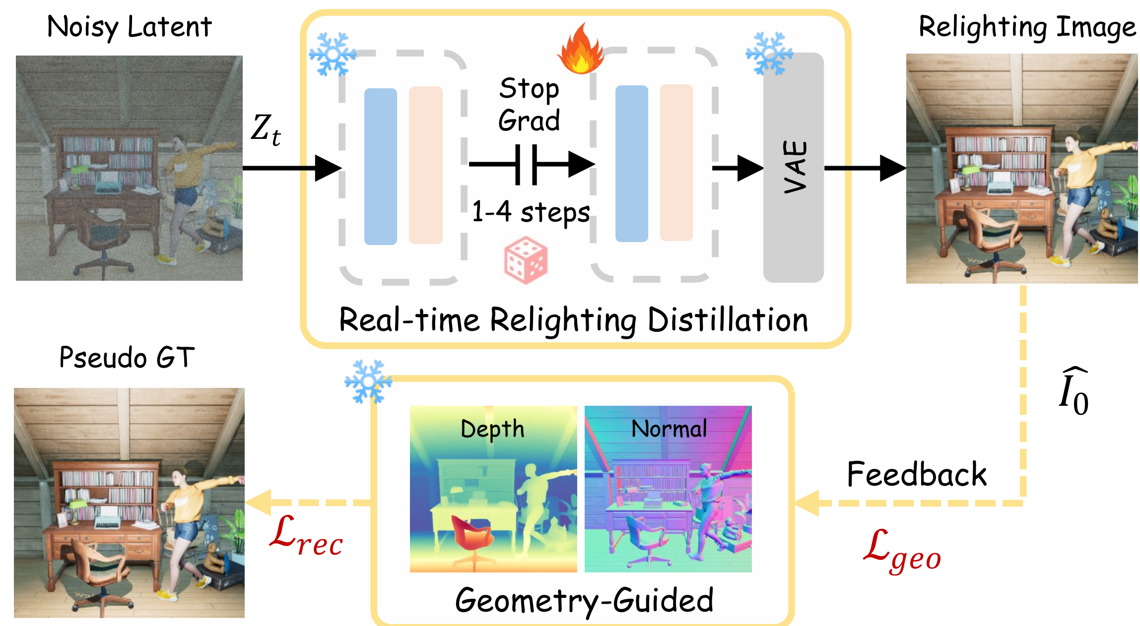
(b) Real-Time Distillation with Geometric Constraints
